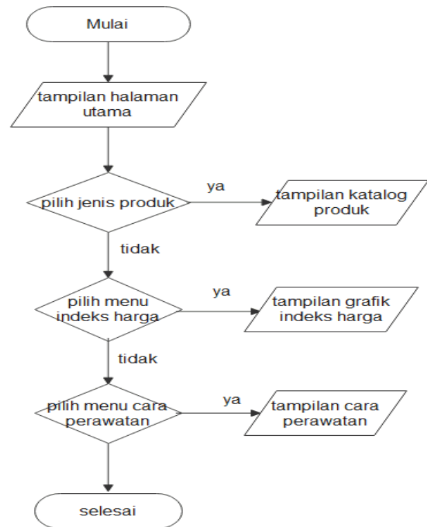
Gambar 3.1 Flowchart Sistem
